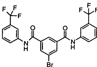
Compound # 26
